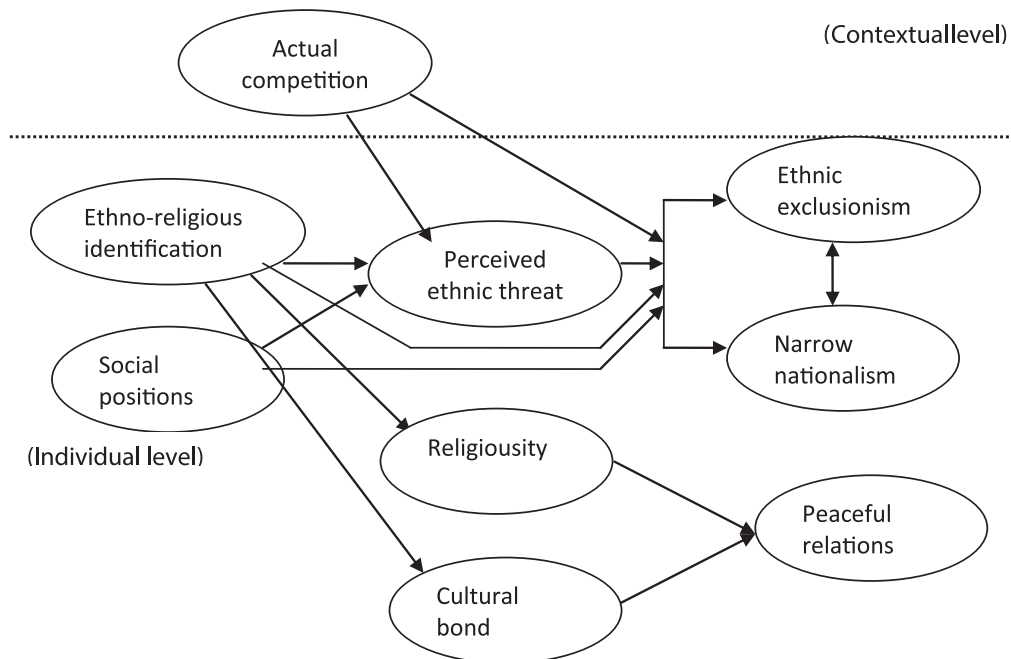
Figure 2.1 Ethnic competition theory: theoretical-conceptual model
